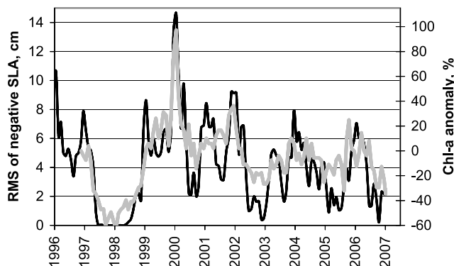
Figure 3. (top) Scatter plot and (bottom) time series of monthly mean RMS of negative SLA (black line, left axis) and Chl-a anomaly (gray line, right axis) in area CRD of Figure 1b.
