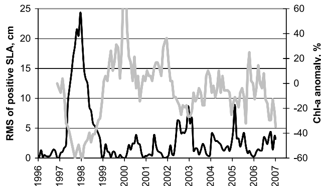
Figure 4. (top) Scatter plot and (bottom) time series of monthly mean RMS of positive SLA (black line, left axis) and Chl-a anomaly (gray line, right axis) in area CRD of Figure 1b.
